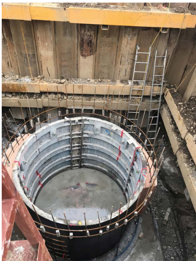
Figure 6: Upgrading the sewer network at Mallow, Co. Cork
